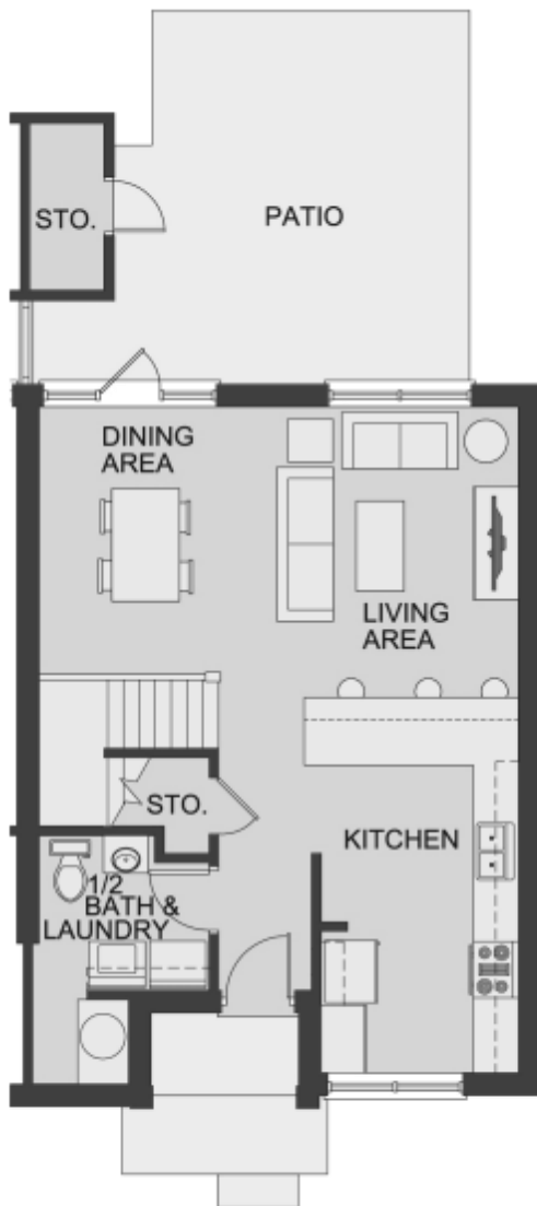
1st Floor
