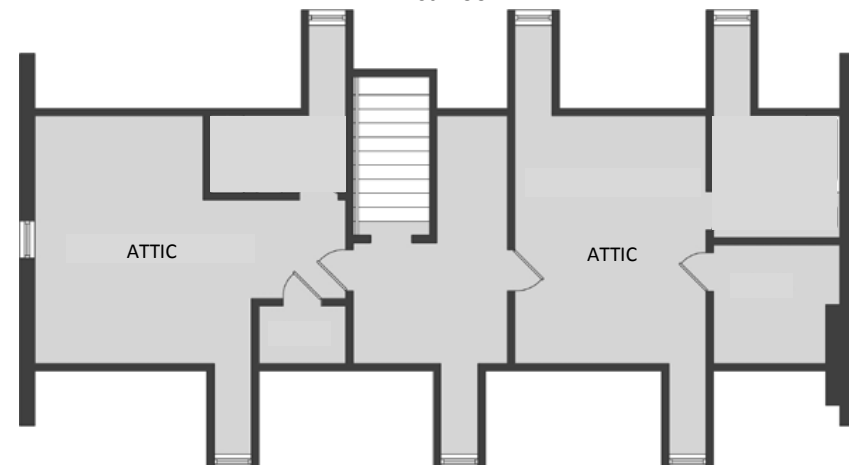
3rd Floor
